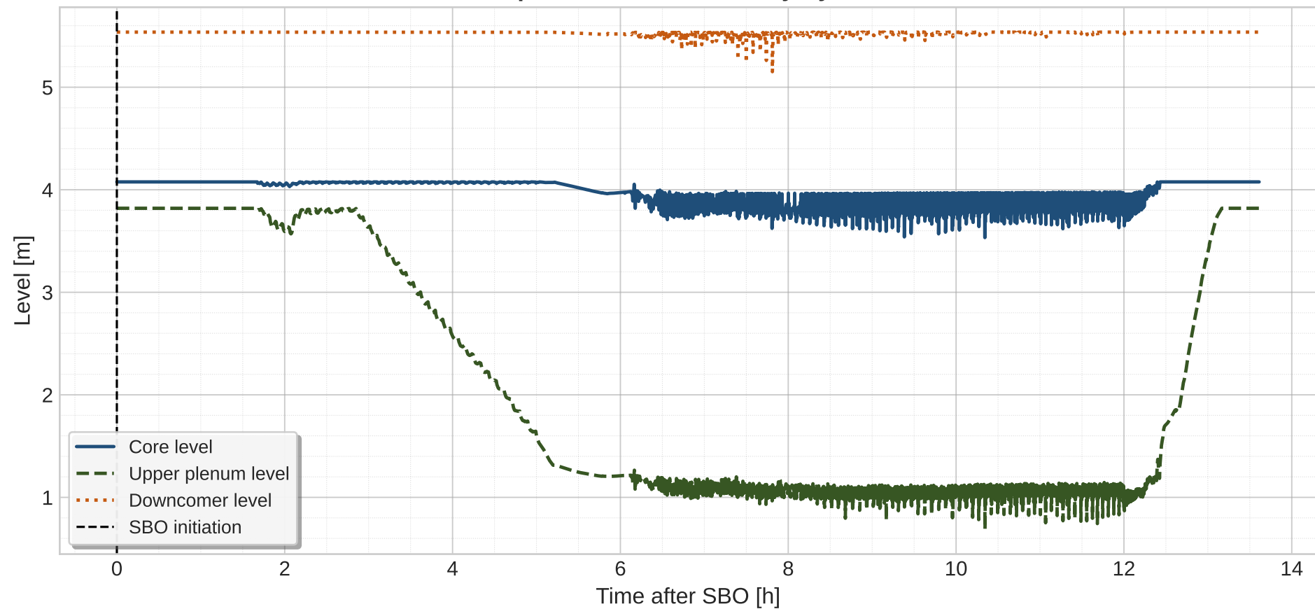
No SG Depressurization - Primary System Levels
